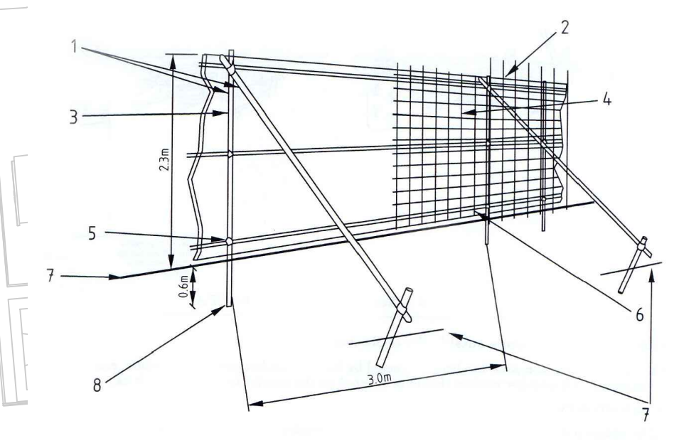
The above displays an example of a suitable protective barrier as recommended by BS. 5837 2012 Trees in Relation to Construction
